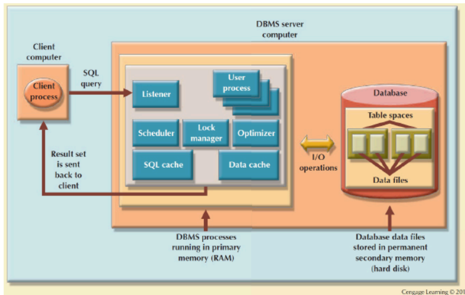
Figure 11.1 - Basic DBMS Architecture
